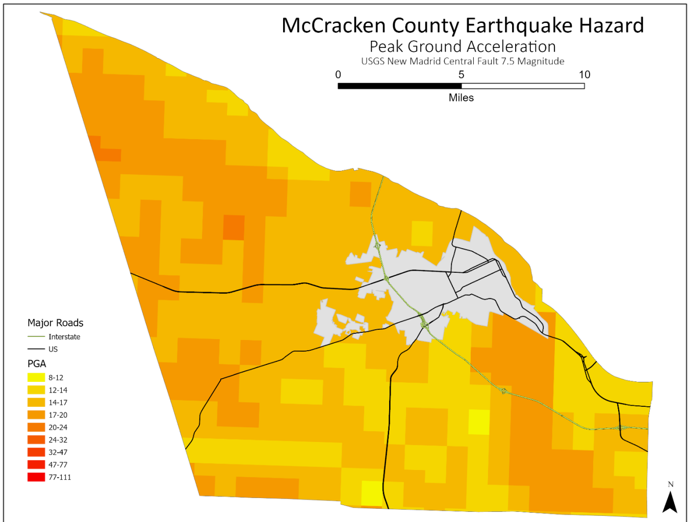
Figure 9.4 USGS New Madrid Central Fault 7.5 Magnitude Peak Ground Acceleration
