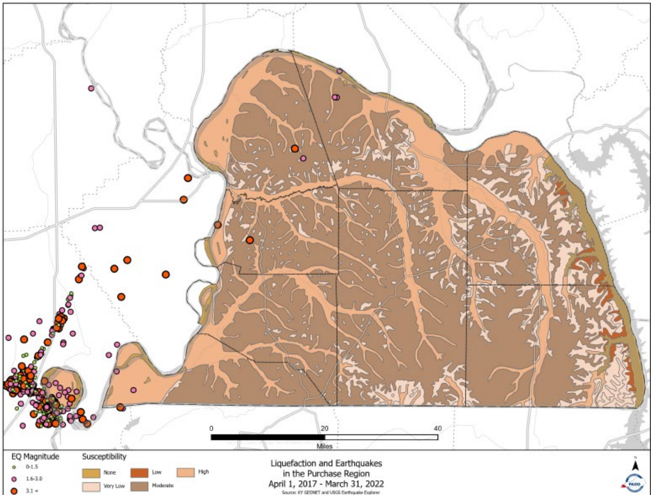
Figure 9.6 Generalized Liquefaction Susceptibility & Earthquake Magnitude of the Purchase Region
