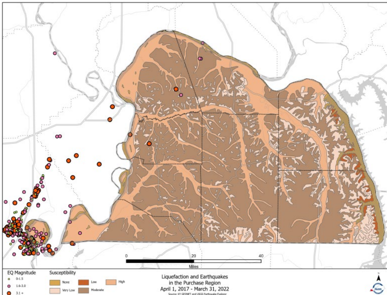
Figure 4.7 Generalized Liquefaction Susceptibility & Earthquake Magnitude of the Purchase Region
