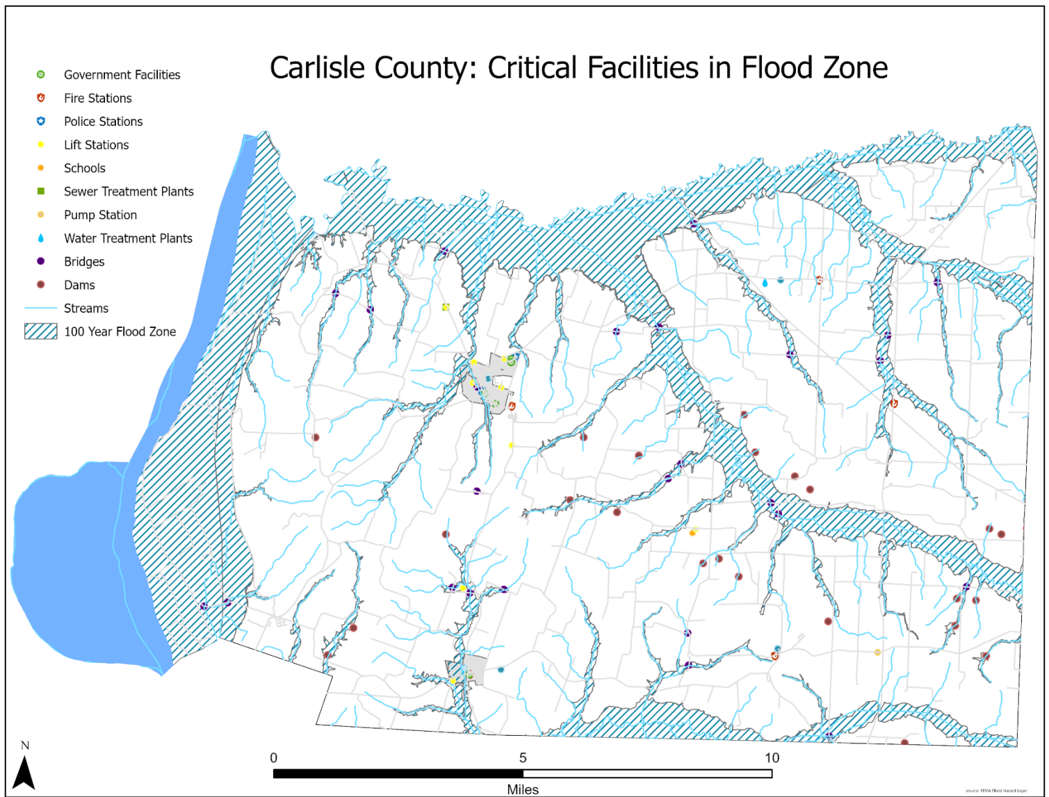
Figure 4.11 Carlisle County Flood Zone Including Critical Facilities
